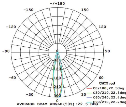
Part Number: KB-H18-45PF-3030 +3030 Led tested
