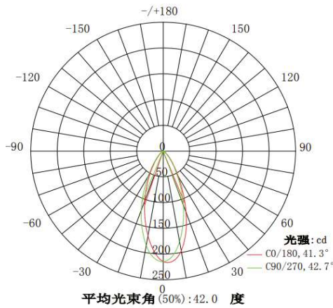
Part Number: KB-H18-2045F-5050 +XPE2 led test
