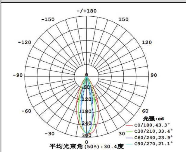
Part Number: KB-H18-2045F-5050 +XPE2 led test
