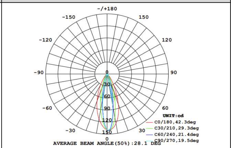
Part Number: KB-H18-2045F-3030 +3030 led tested
