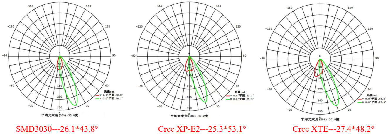
Part Number: KB-H20-1530-3030-SC/HC
