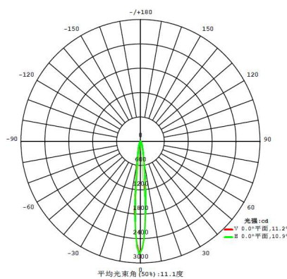
Part Number: KB-H20-12P-3030-SC/HC
