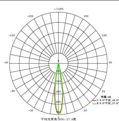
Part Number: KB-H20-20P-3030-SC/HC
